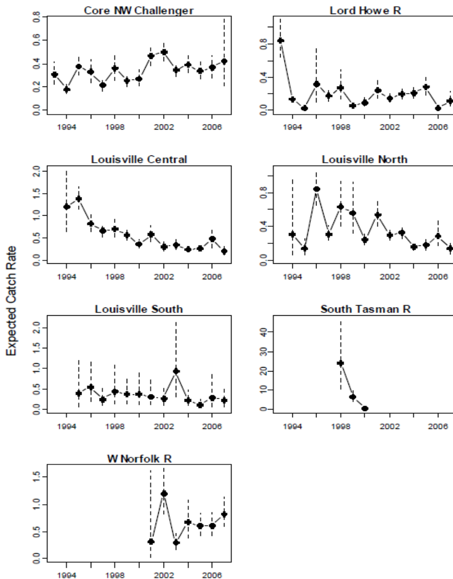
Figure 4. Standardised CPUE trends (model prediction fishing year effects) for orange roughy by fishing area outside of the EEZ, made with all other predictors set to the median (fixed) values. (Clark et al. 2010)
