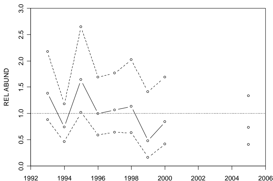
Figure 29: Time series of relative abundance estimates based on January and February (not March), with 90% confidence intervals (from Bravington et al 2005).
