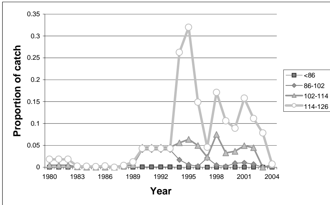
Figure 23: New Zealand domestic SBT catch estimated size/age composition. For discussion, we assume that fish of size <86cm correspond to age-classes 0-2, 86-102 cm = age 3; 102-114 cm = age 4 and 114-126 cm = age 5.
